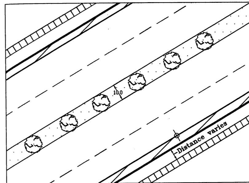
Typical Section
